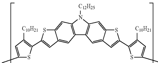
Comparative compound 4
