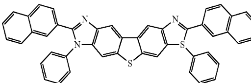
Comparative compound 4
