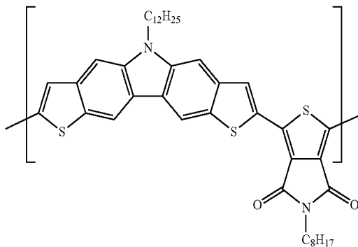
Comparative compound 3
